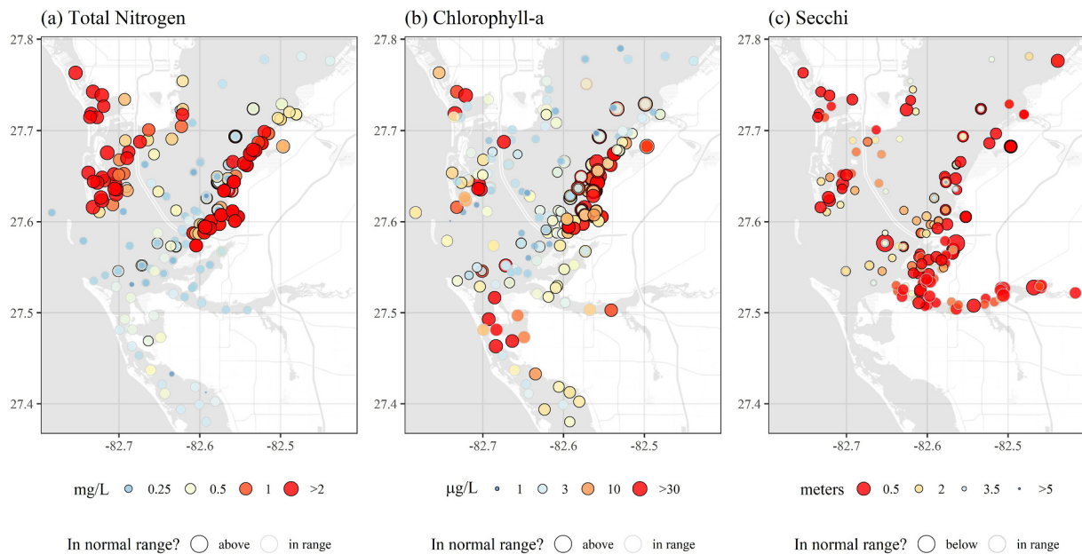
Fig. 2. Water quality data (raw observations) for April through September 2021 following the release from Piney Point for (a) total nitrogen (mg/L), (b) chlorophyll-a (µg/L), and (c) Secchi disk depth (meters). Values outside of the normal range (above for total nitrogen and chlorophyll-a, below for Secchi) are outlined in black and those in normal range are outlined in light grey. Color ramps and point sizes show relative values (reversed for Secchi). Normal ranges are defined as within \pm 1 standard deviation of the mean for the month of observation from 2006 to 2020 for values collected at the nearest long-term monitoring site to each sample location (Fig. 1a). Values below detection limits (or Secchi on bottom) are not shown. (For interpretation of the references to color in this figure legend, the reader is referred to the web version of this article.)
