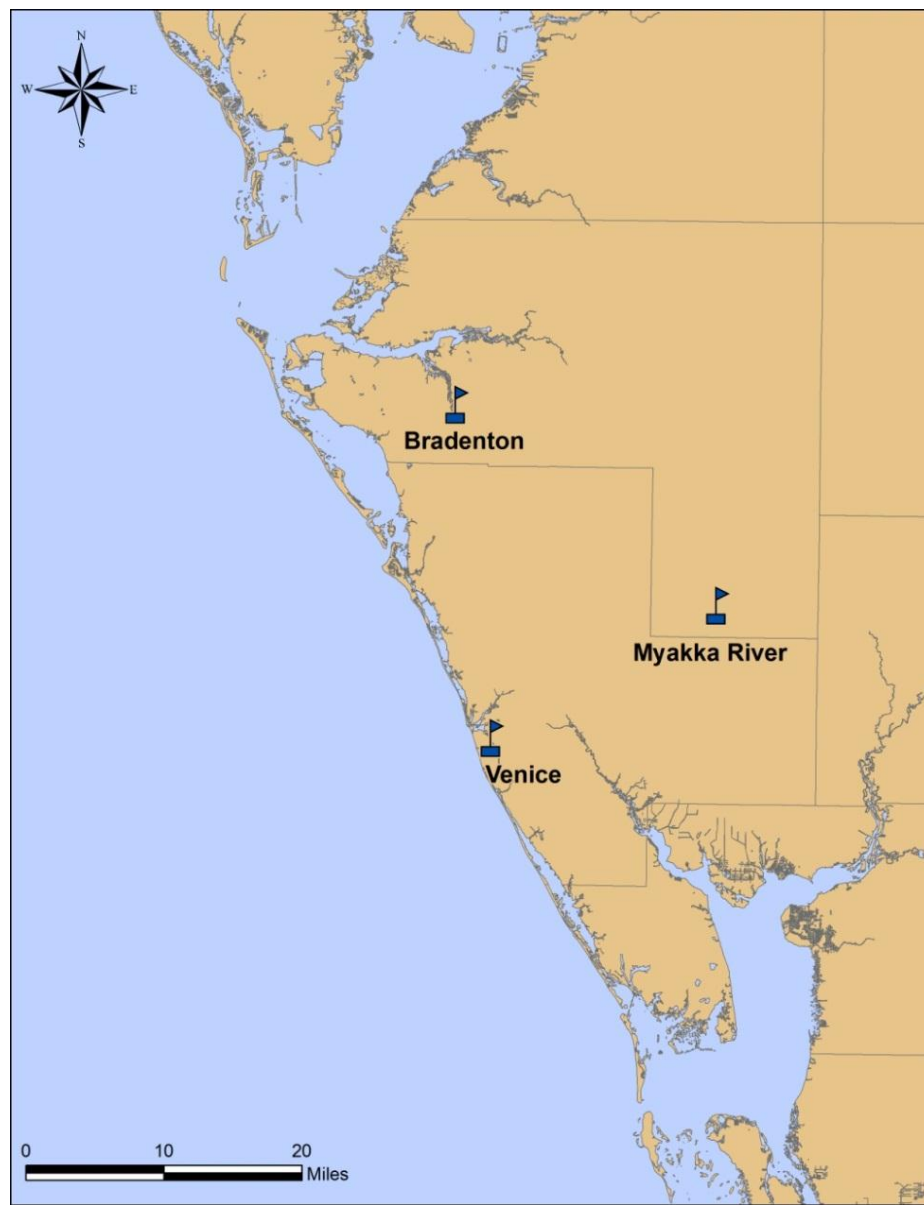
Figure 6. Location of long-term rain gauges used in compliance assessment.
