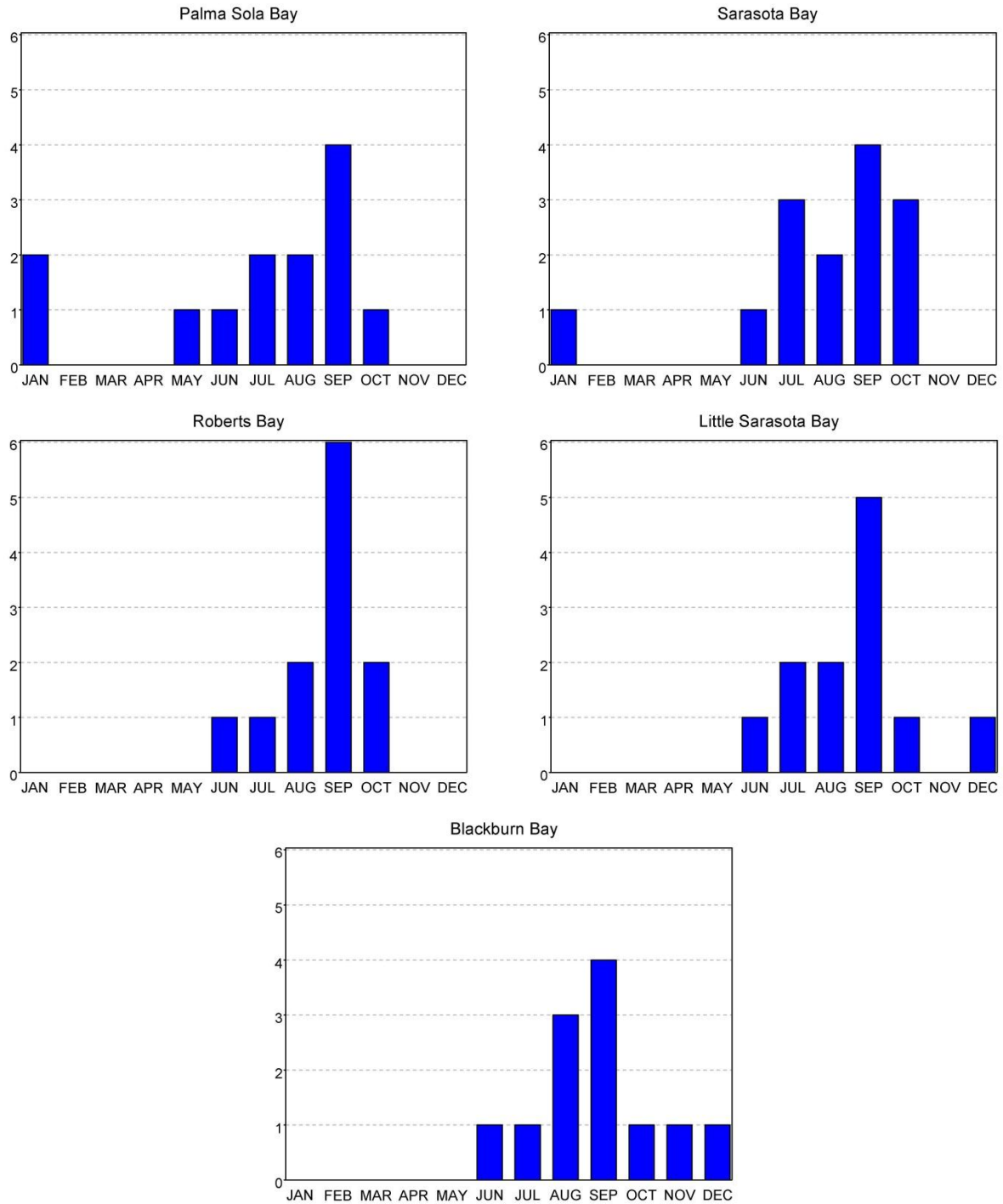
Figure 4. Number of occurrences within each month of maximum chlorophyll a.
