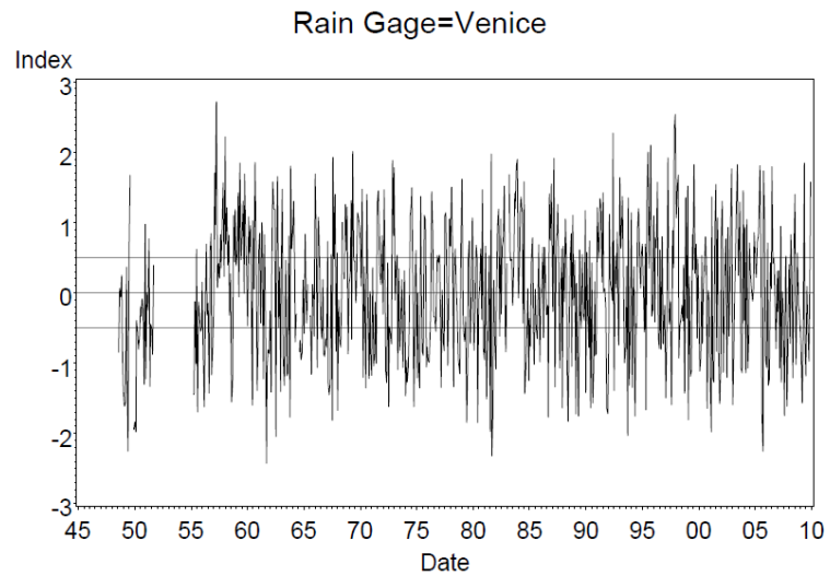
Figure 7. Time series of monthly rainfall values standardized to their long-term monthly average.
