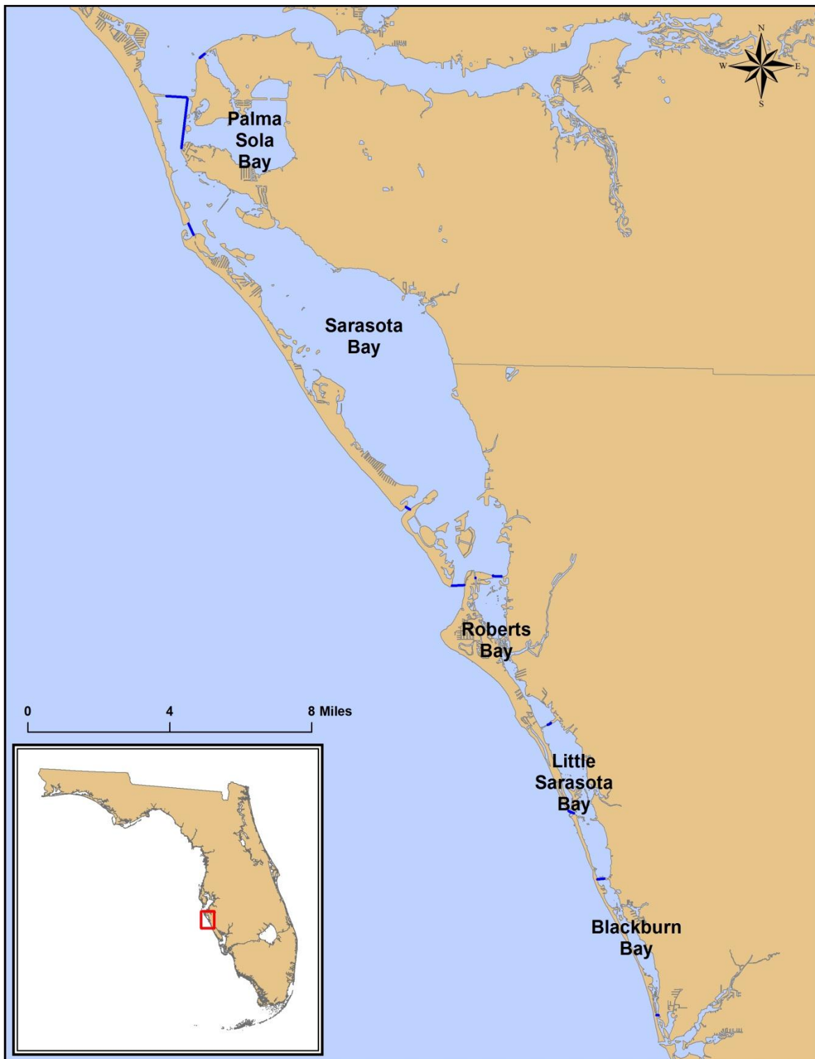
Figure 1. Bay segments within the Sarasota Bay Estuary Program system.
