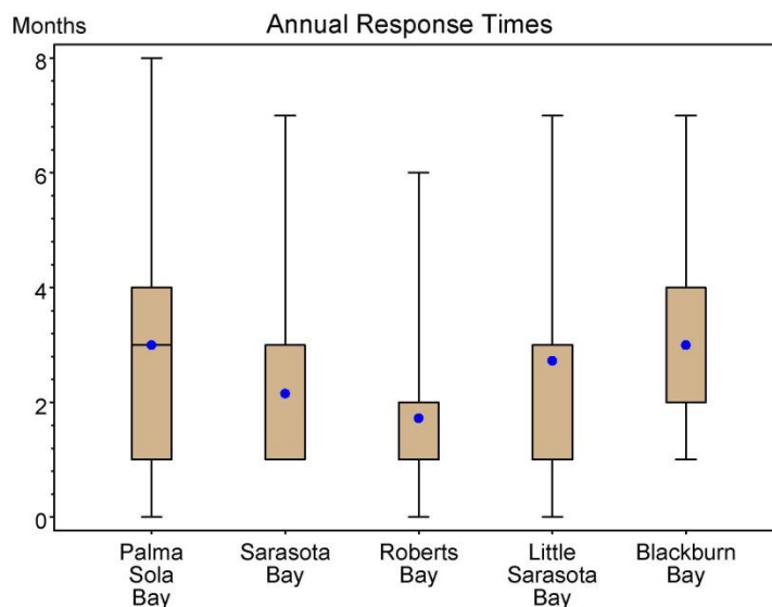
Figure 3. Annual chlorophyll a response times (months) for the period 1997-2008.
