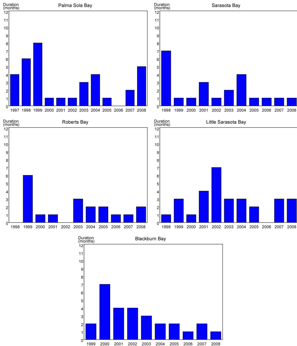
Figure 5. Recovery period (months) to return from annual maximum chlorophyll a to below monthly median value.
