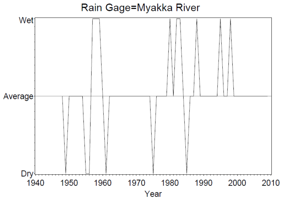
Figure 9. Results of annual classification of rainfall data anomalies for the Myakka River rain gage.
