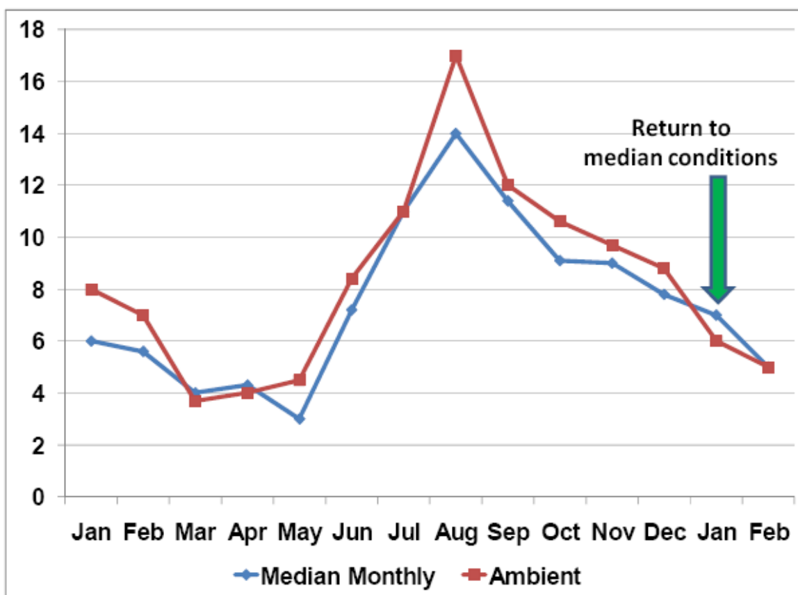
Figure 2. Example of the response time estimation method.
