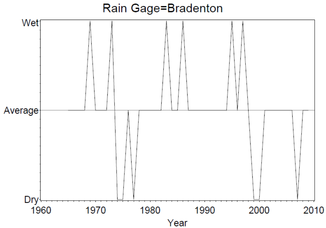
Figure 8. Results of annual classification of rainfall data anomalies for the Bradenton Rain gage.
