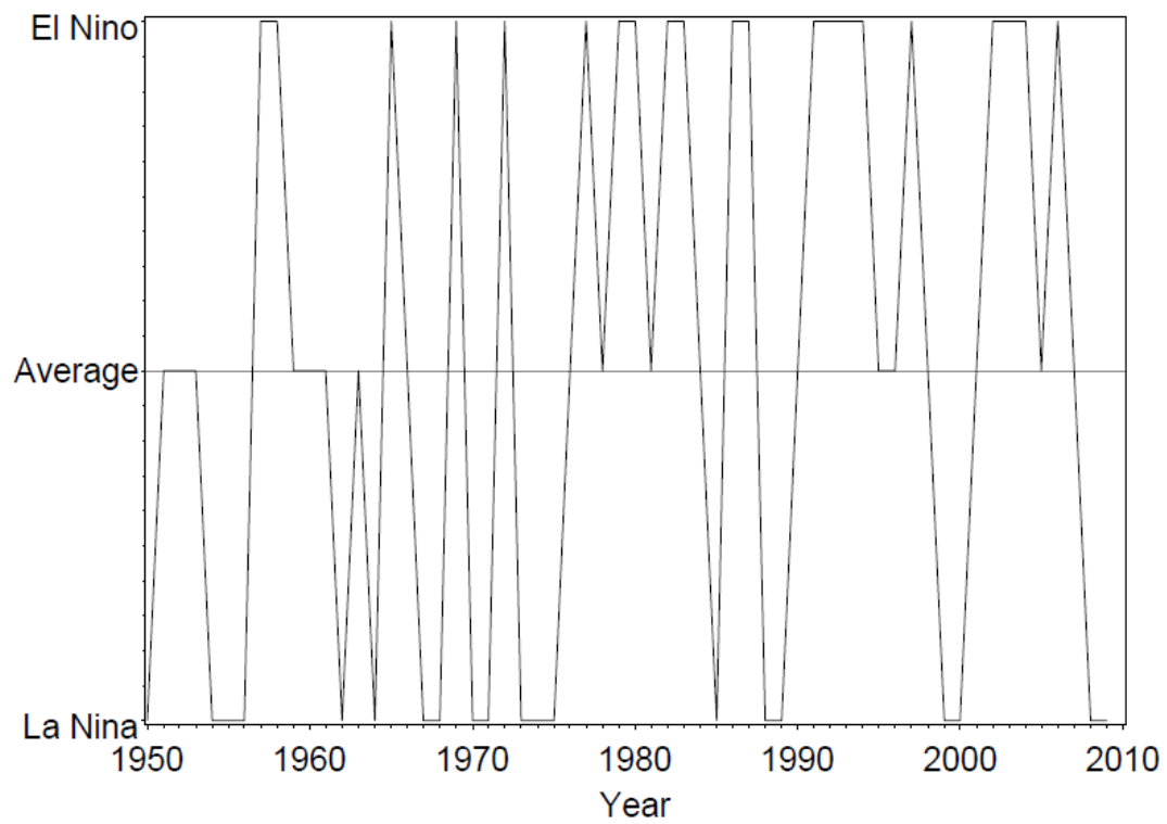
Figure 11. Results of annual classification of ENSO MEI data anomalies 1950-2008.
