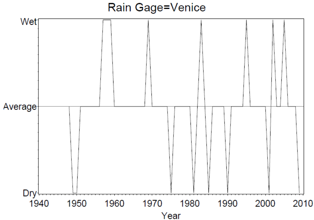
Figure 10. Results of annual classification of rainfall data anomalies for the Venice rain gage.
